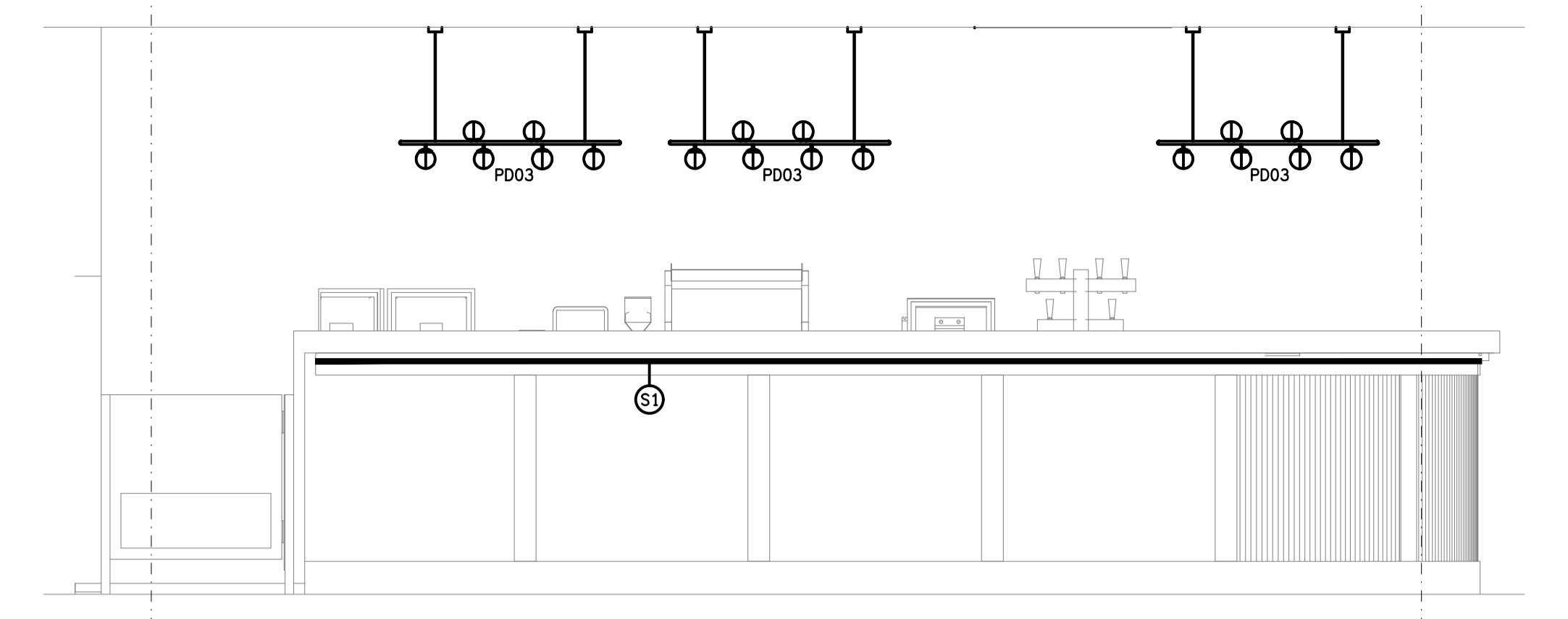
DETAIL A GAMING FRONT COUNTER ELEVATION SCALE 1:25
